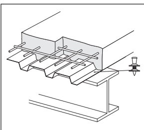
Floor decking
