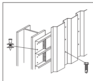
Wall liners
