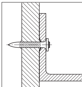
Angle bracket
